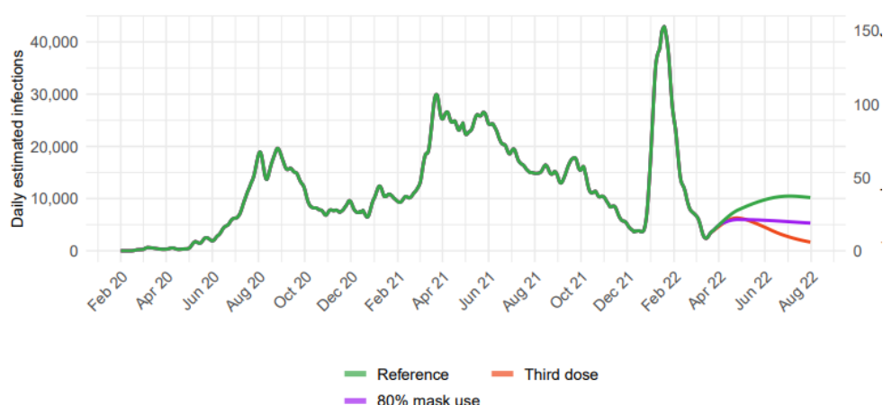
Figure 22.1: Daily COVID-19 infections until August 01, 2022 for three scenarios
