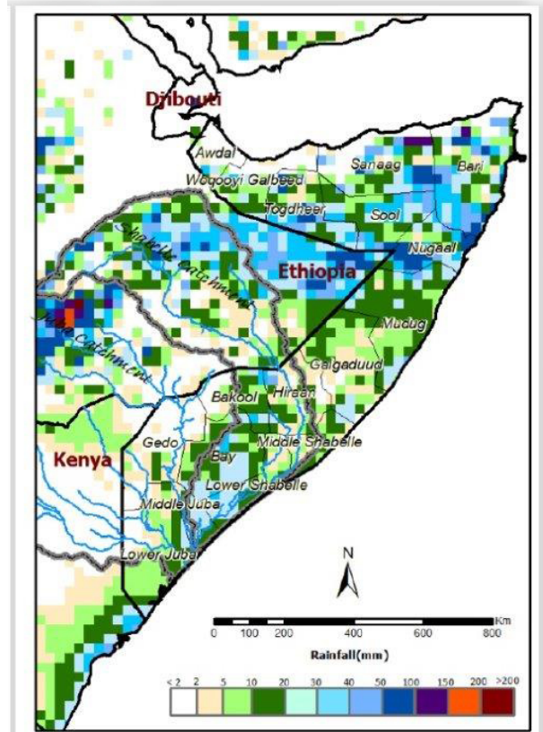
7-day cumulated rainfall forecast (27 Sept to 03 Oct 2018)
