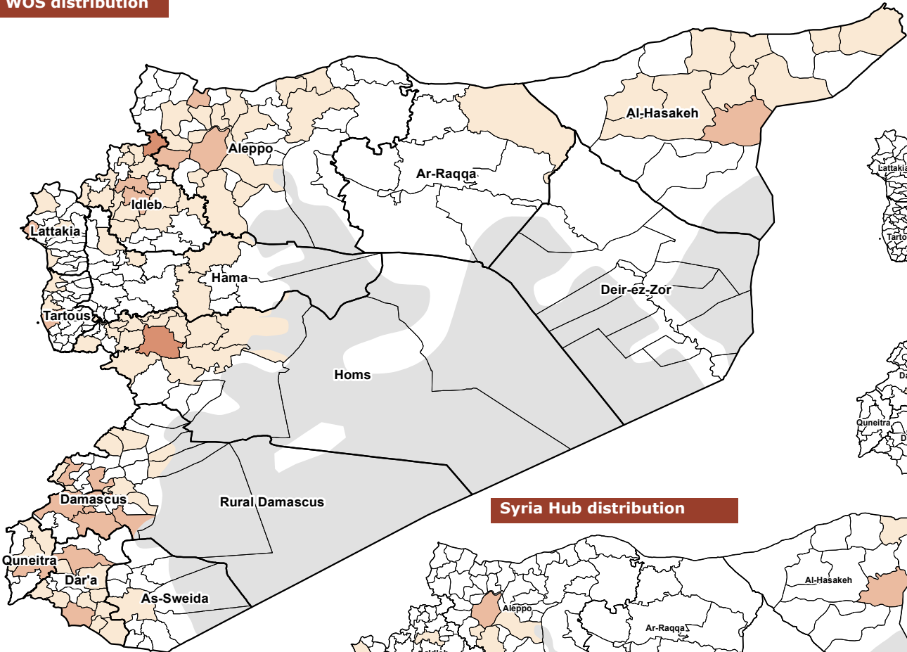
WOS distribution
