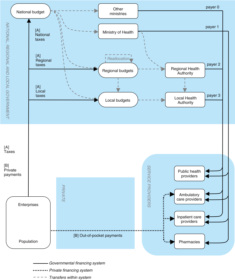
Fig. 3.6 Financial flows, 2013
